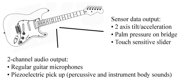
Figure 2. The CICM augmented electric guitar set-up
